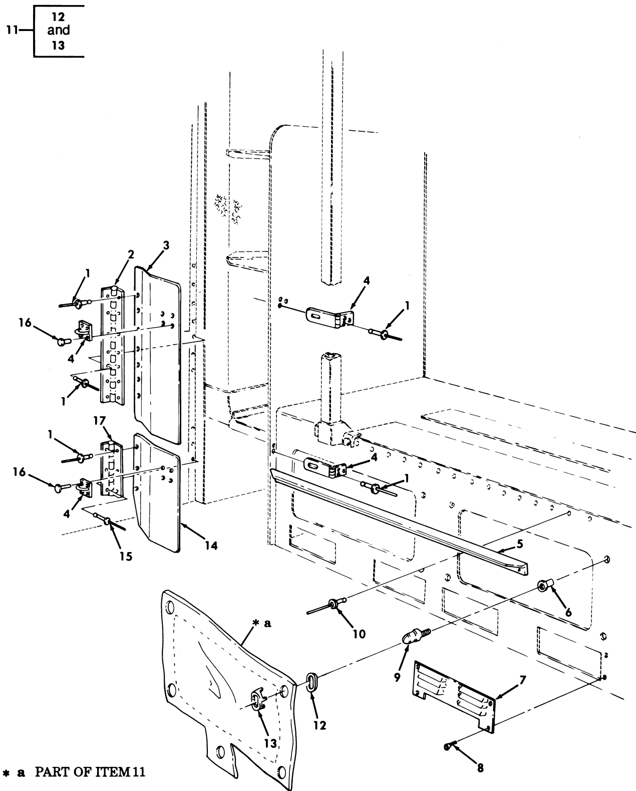
Figure 224. Medical Stowage Doors, Lower Heater Louver, and Related Components, M997, M997A1, and M997A2 Ambulance.
