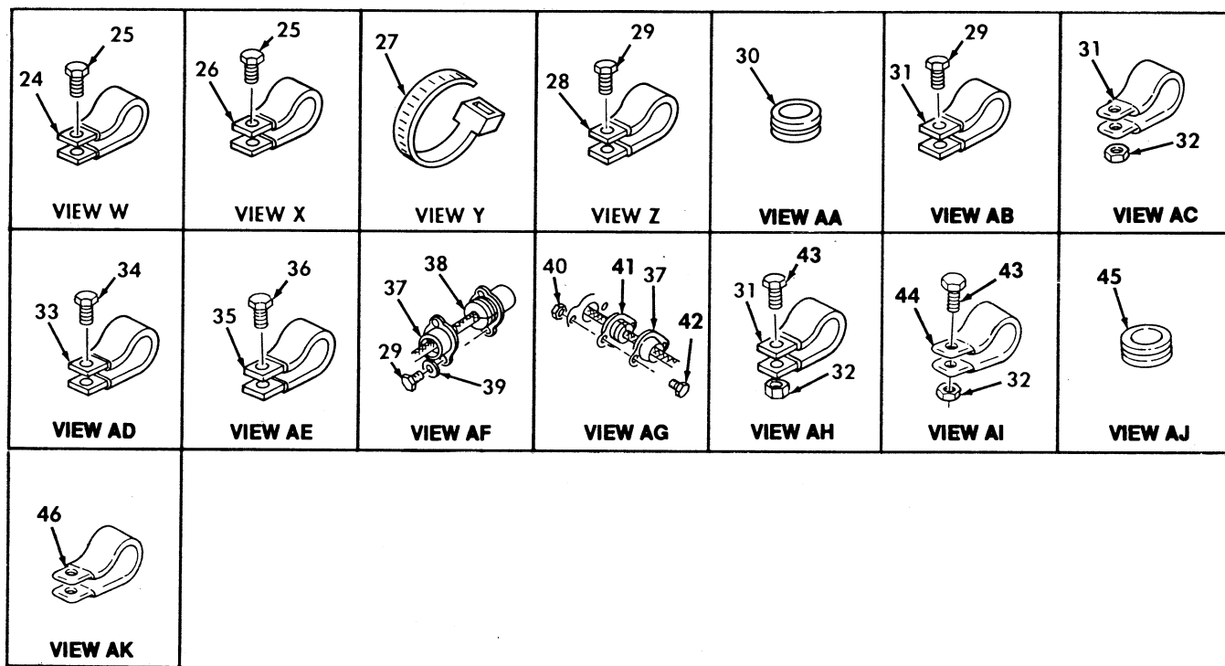
Figure 95. NBC Wiring Harness, M997, M997A1, and M997A2 Ambulance (Sheet 1 of 2).
