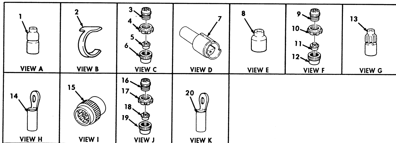
Figure 86. A2 Body Wiring Harness (Sheet 1 of 2).
