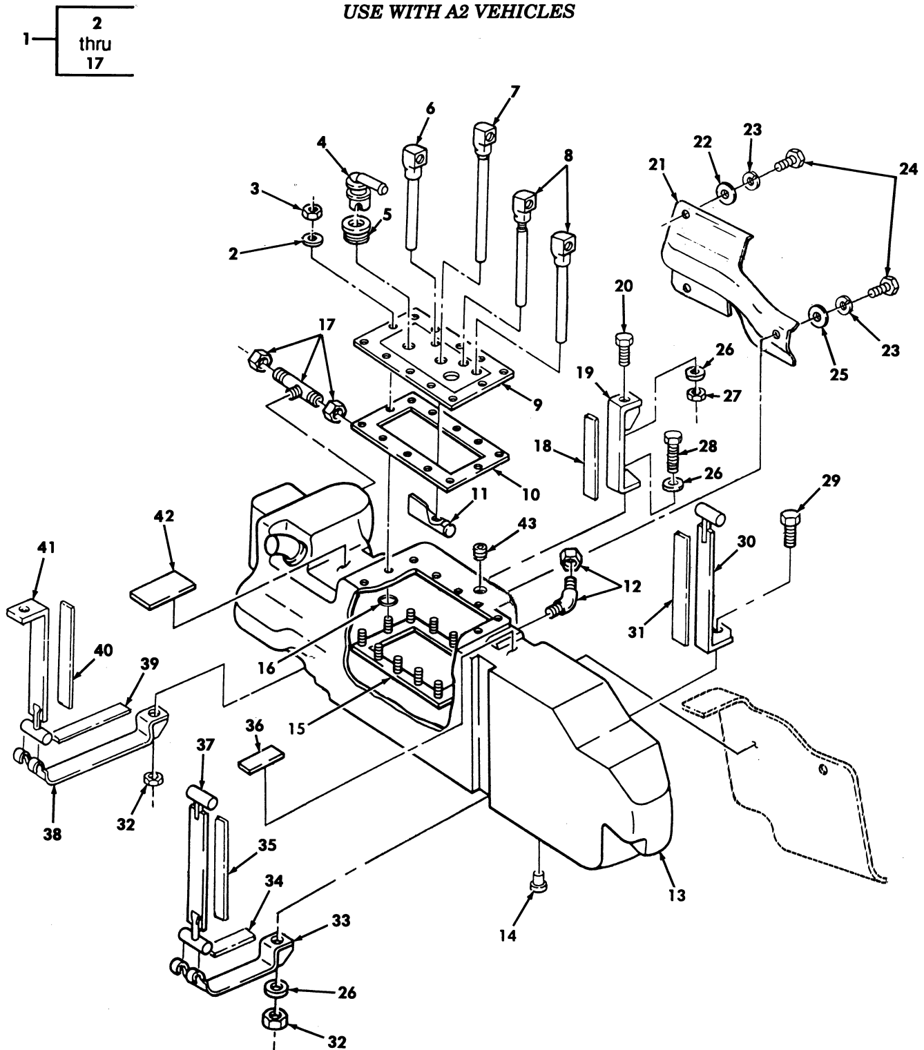
Figure 16. Fuel Tank Assembly and Mounting Straps.
