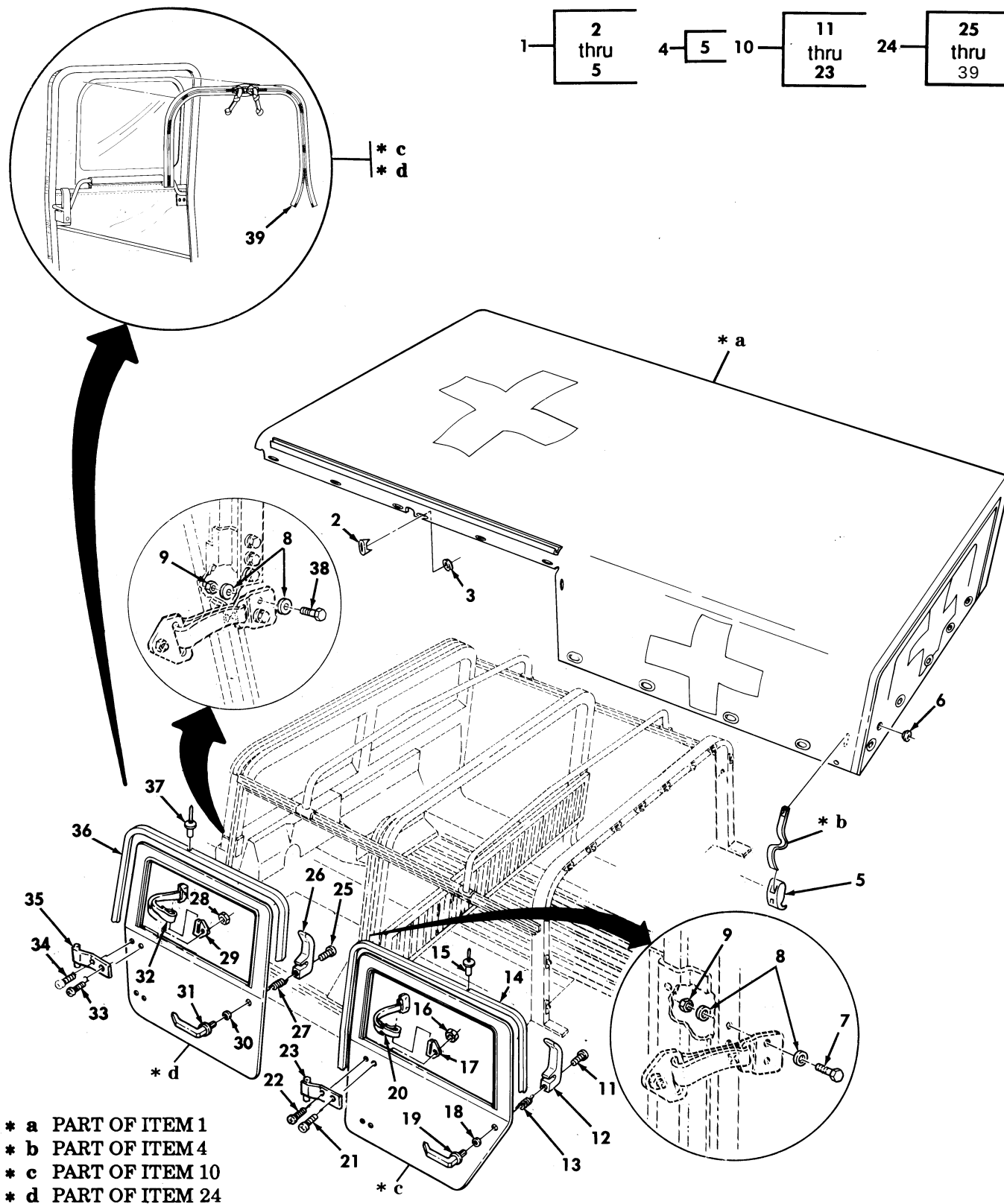
Figure 324. Ambulance Soft Top Enclosure, Top Curtain, and Door Assemblies.
