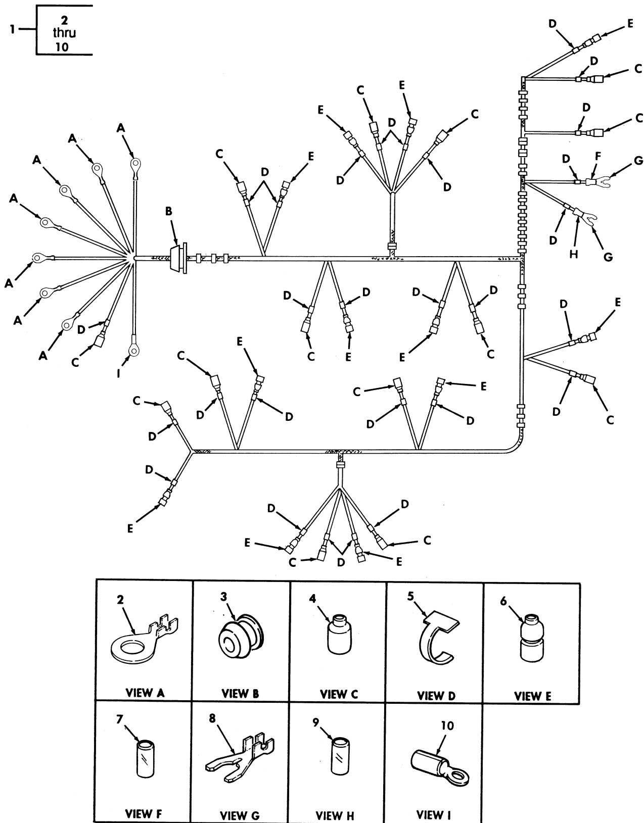
Figure 92. Interior Lighting Harness Assembly, M996, M996A1, M997, M997A1, and M997A2 Ambulance (Sheet 1 of 2).
