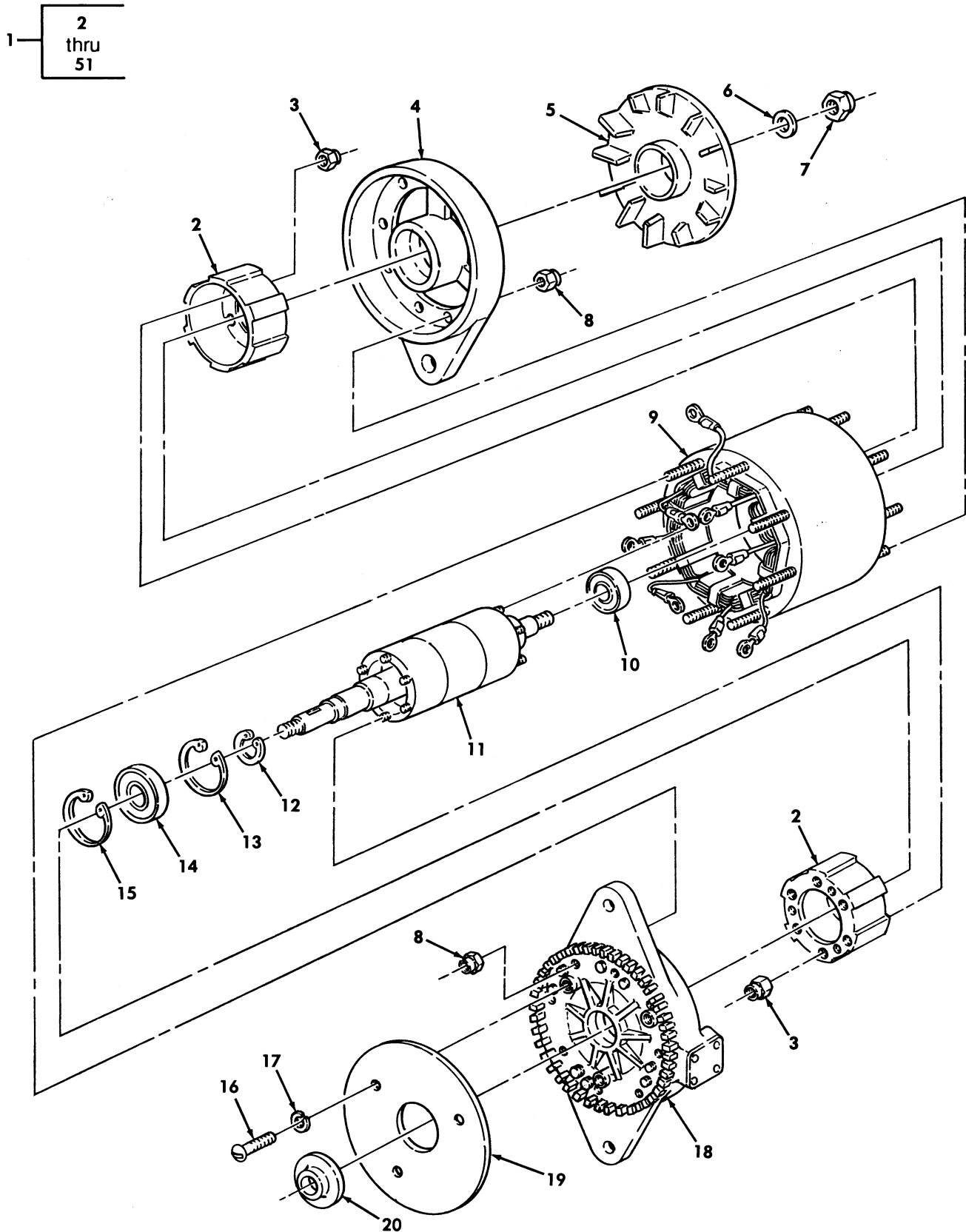
Figure 40. 200 AMP Alternator, M996, M996A1, M997, M997A1, M997A2, M1025A2, M1035A2, M1043A2, M1045A2, M1097, M1097A1, M1097A2, and M1123 (NIEHOFF) (Sheet 1 of 2).
