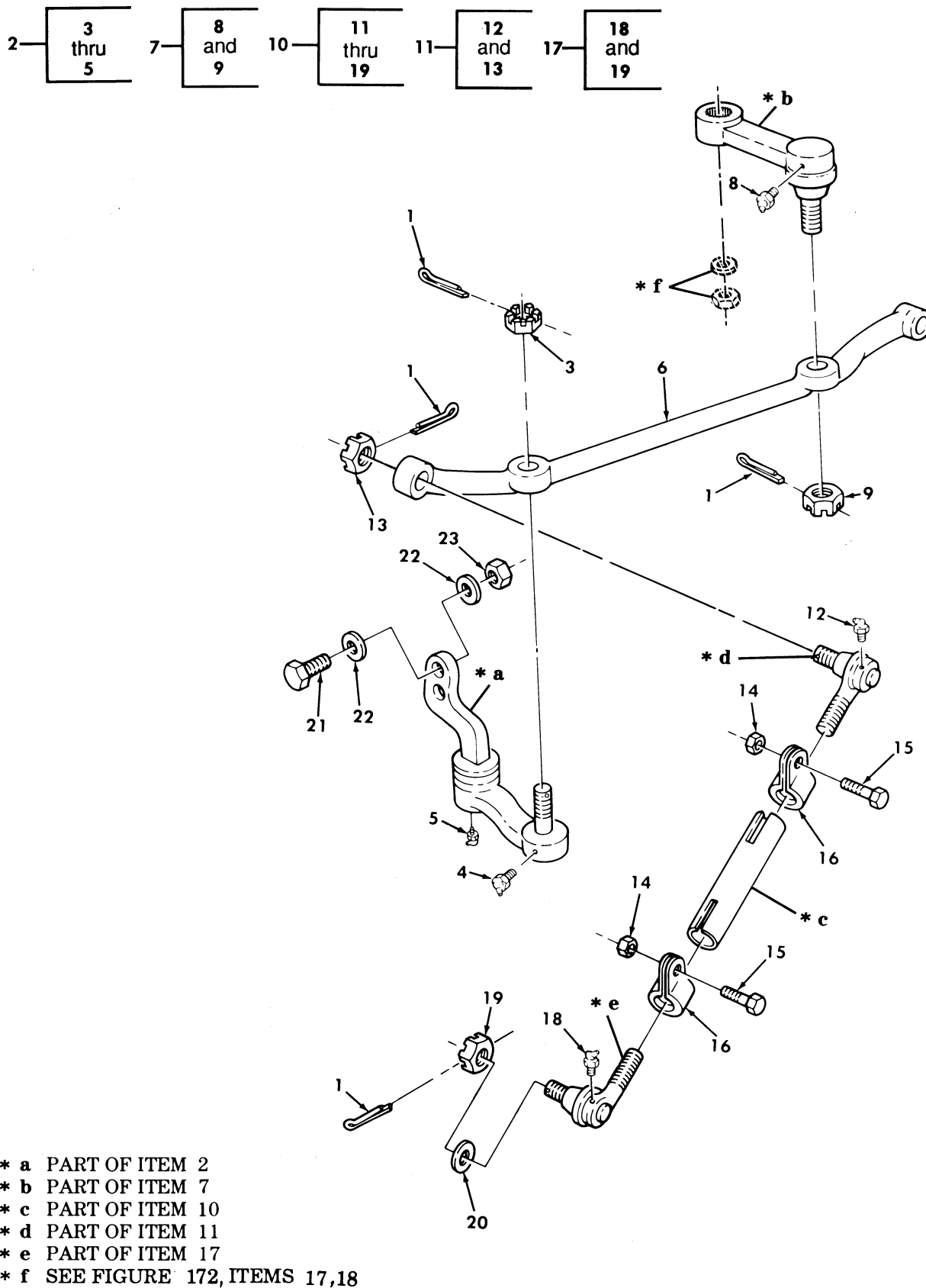
Figure 170. Steering Linkage.
