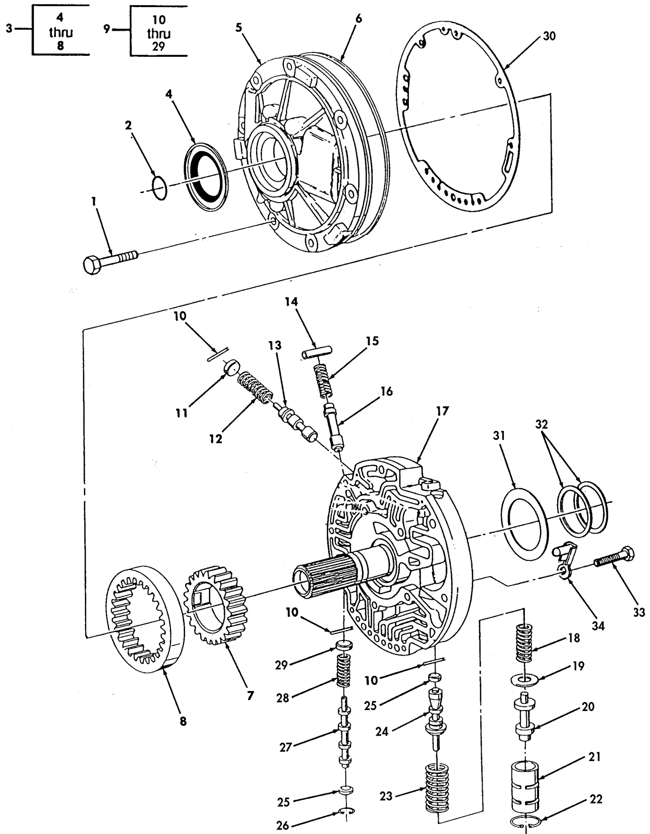
Figure 122. Transmission Oil Pump.
