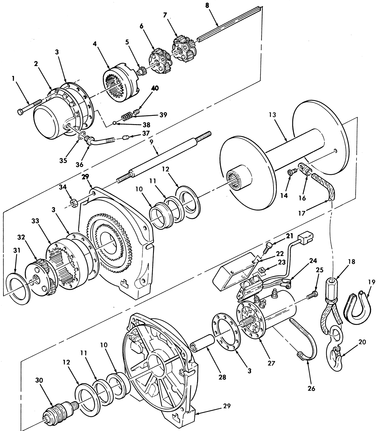
Figure 314. Winch Assembly.
