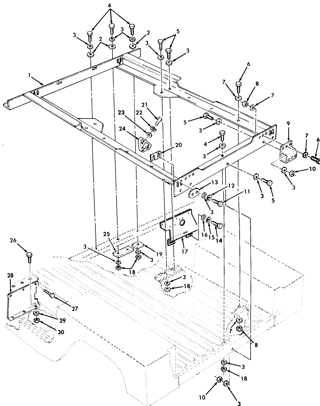
Figure 283. S250 Shelter Mounting Components.
