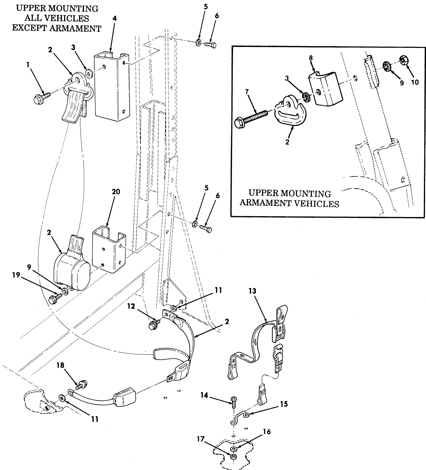
Figure 234. Front Seatbelts, Brackets, and Mounting Hardware.
