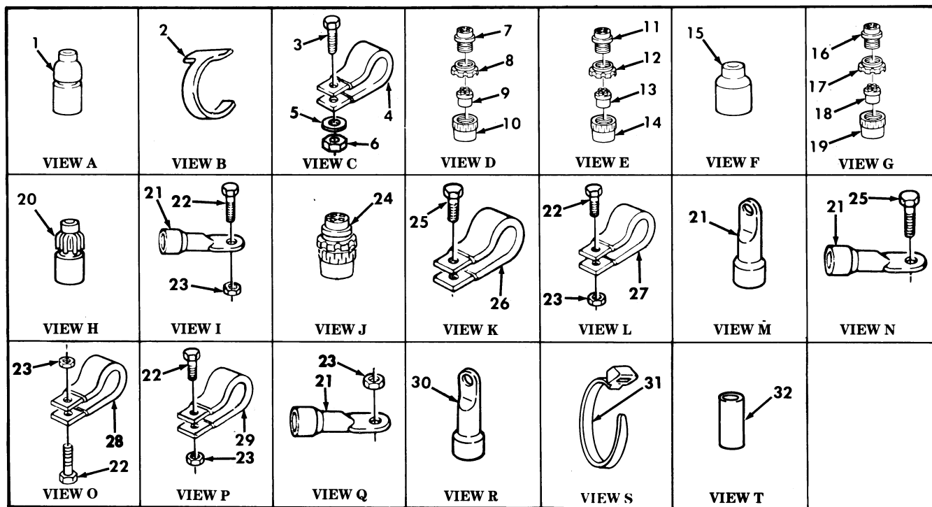
Figure 85. Body Wiring Harness – Partial View.
