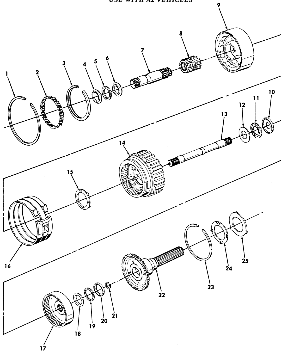
Figure 107. Planetary Gear Carrier.
