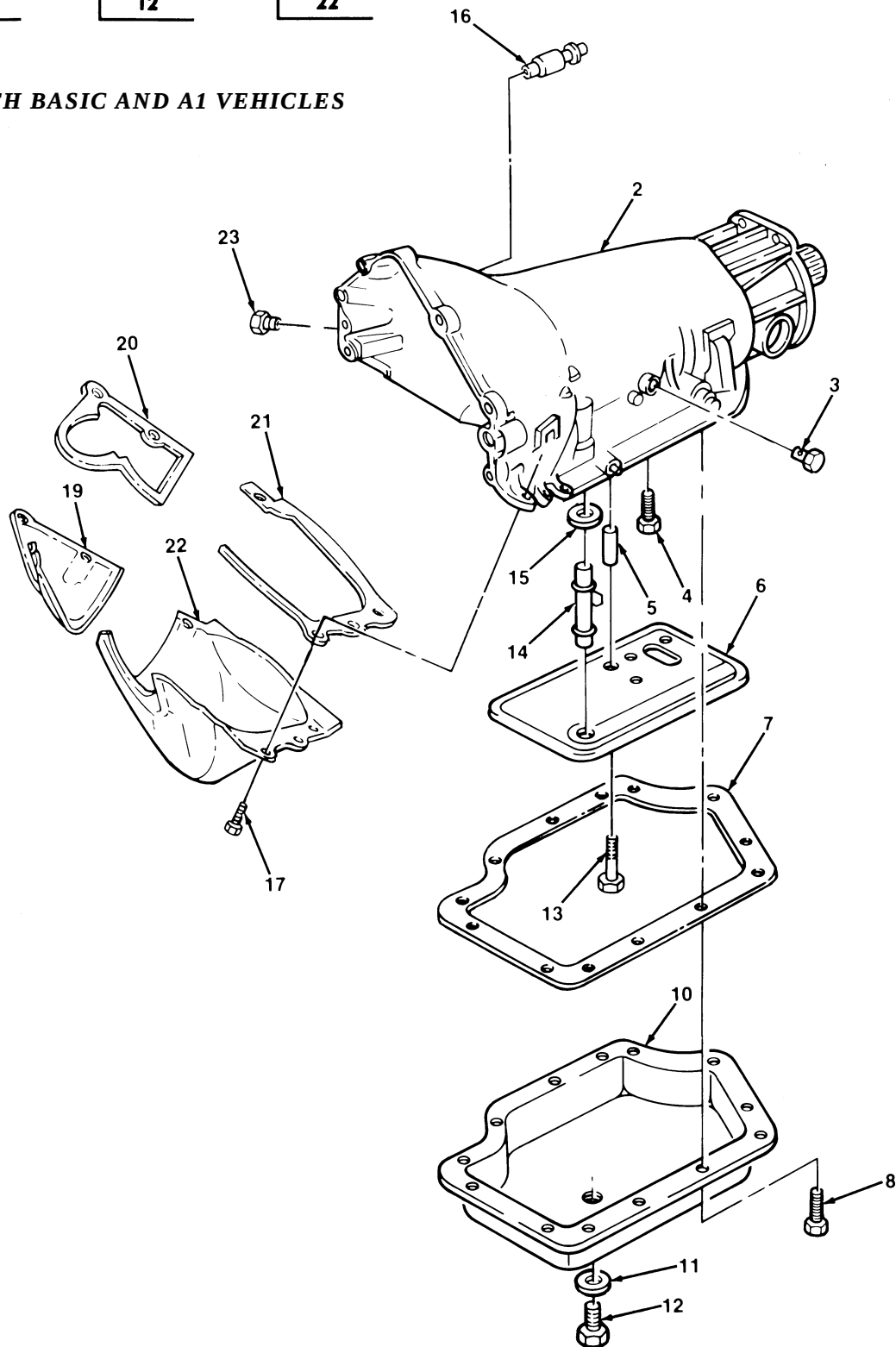
Figure 104. Transmission Assembly.
