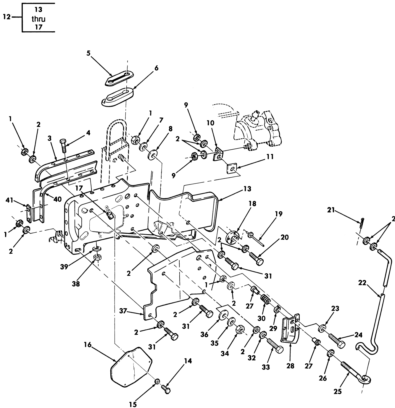
Figure 205. Left Hand Splash Shield, Radiator Side Armor, and Hood Prop Rod.
