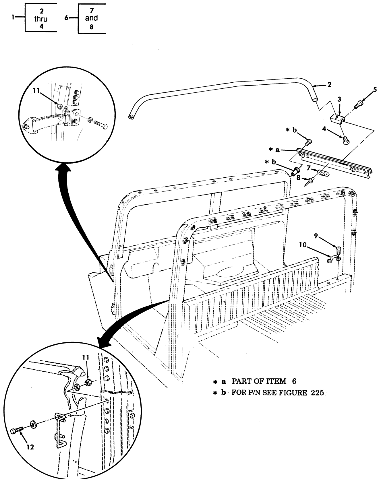
Figure 317. Two Man Crew Soft Top Enclosure, Bow, and Mounting Components.
