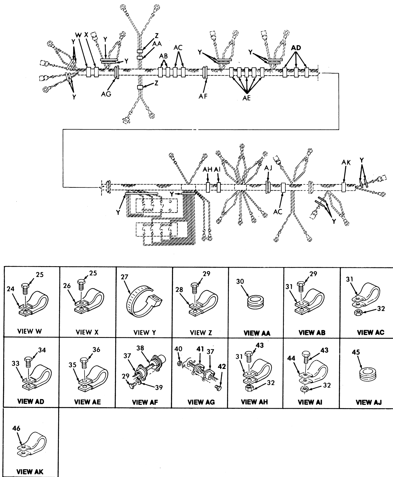
Figure 95. NBC Wiring Harness, M997, M997A1, and M997A2 Ambulance (Sheet 2 of 2).
