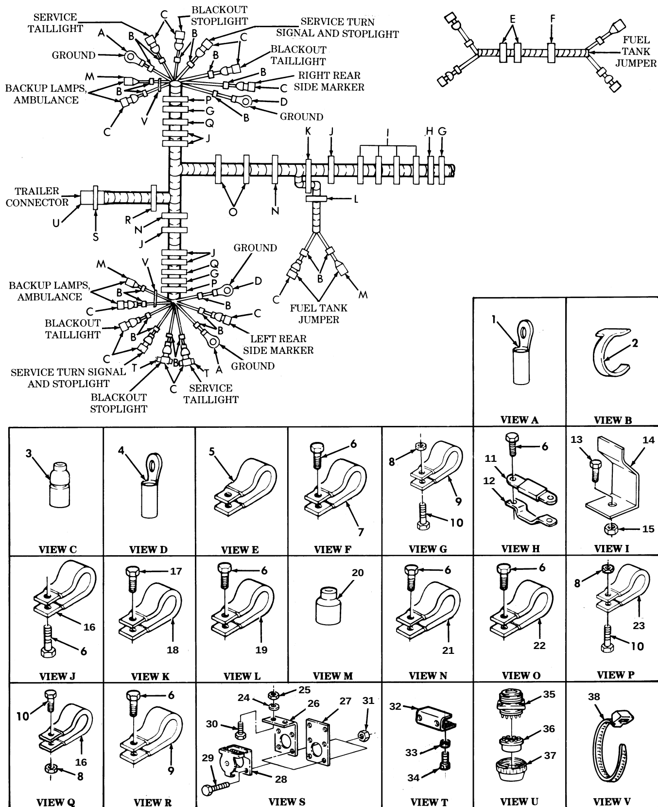
Figure 83. Body Wiring Harness - Partial View.
