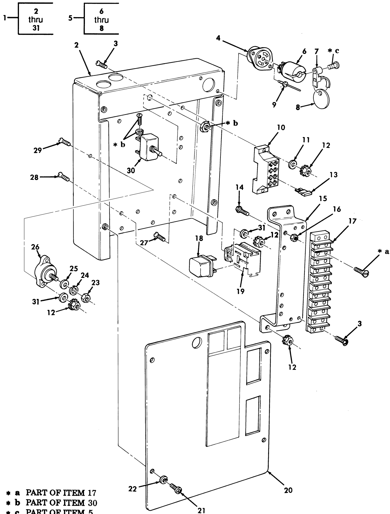
Figure 52. Control Box Assembly, M996, M996A1, M997, M997A1, and M997A2 Ambulance.
