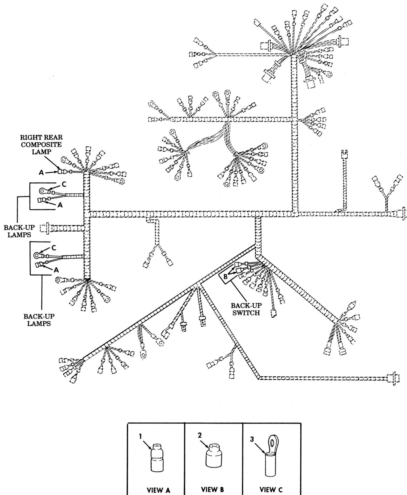
Figure 87. Ambulance Body Wiring Harness, M997A2 and M1035A2 (Sheet 1 of 2).
