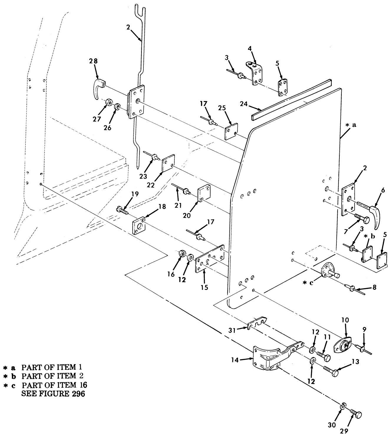
Figure 212. Rear Doors, M997, M997A1, and M997A2 Ambulance.
