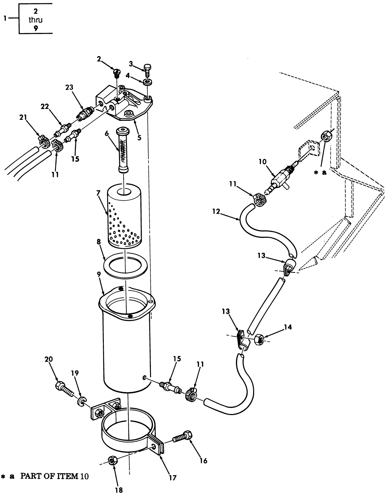
Figure 19. Fuel Filter Assembly/Water Separator and Mounting Hardware.
