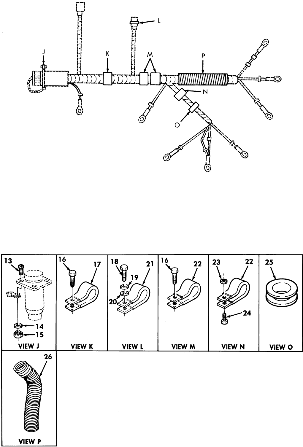
Figure 79. STE/ICE Wiring Harness (Sheet 2 of 2).
