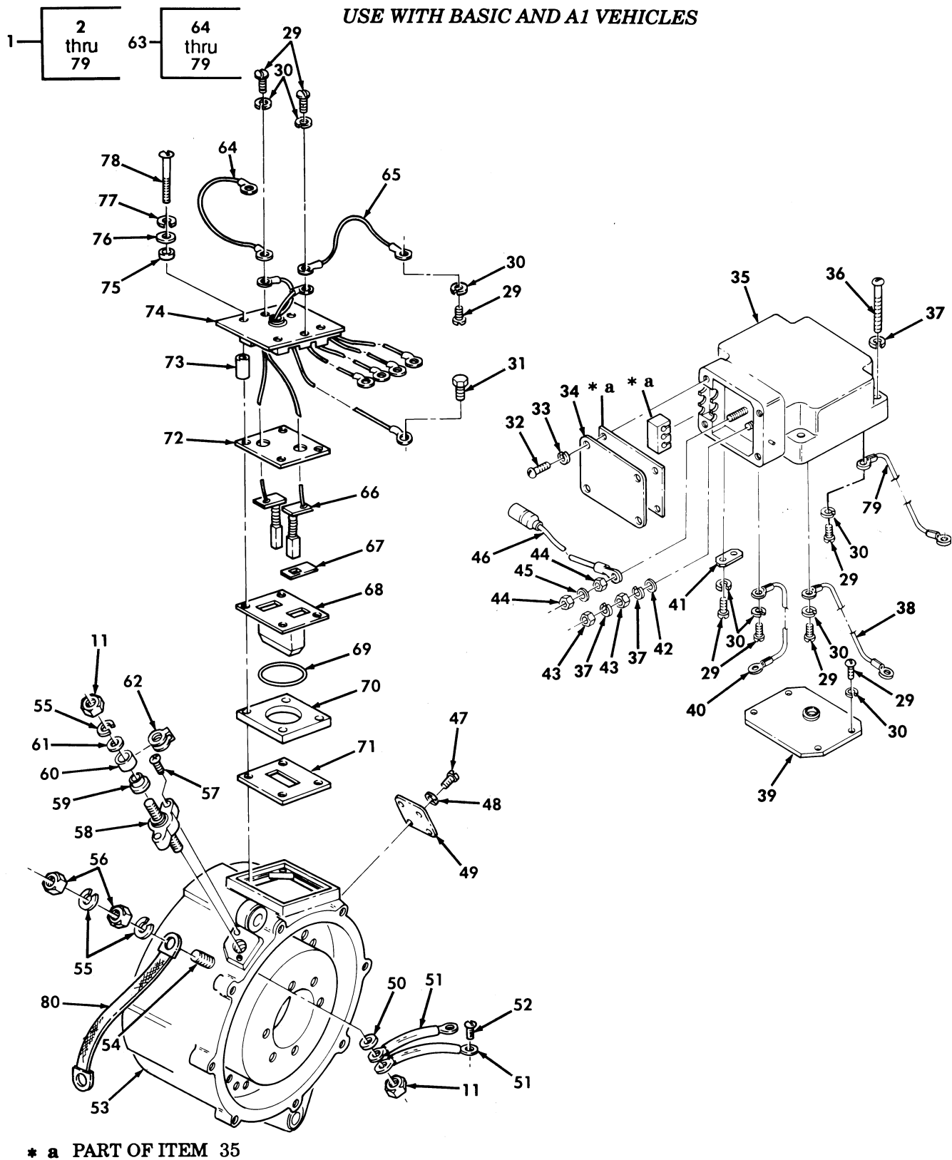
Figure 39. 200 Amp Alternator, M996, M996A1, M997, M997A1, M1097, and M1097A1 (PRESTOLITE) (Sheet 2 of 2).
