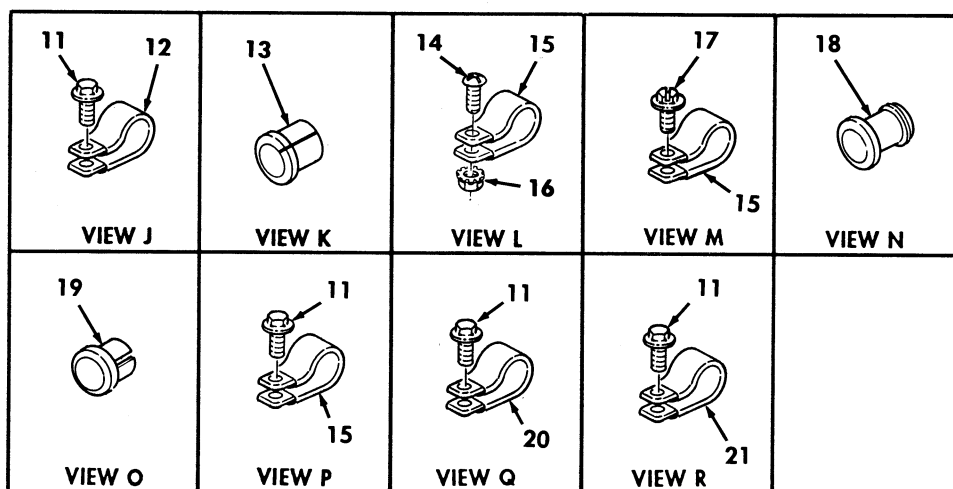
Figure 92. Interior Lighting Harness Assembly, M996, M996A1, M997, M997A1, and M997A2 Ambulance (Sheet 2 of 2).
