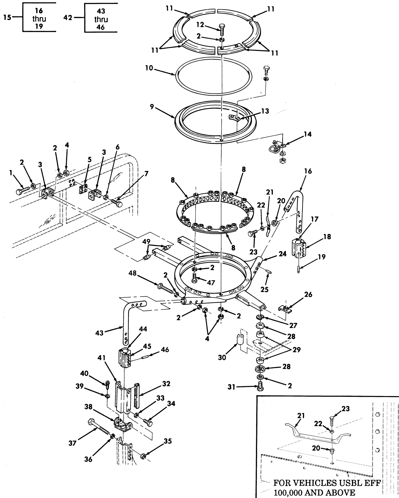
Figure 277. Turret Support Ring Assembly.
