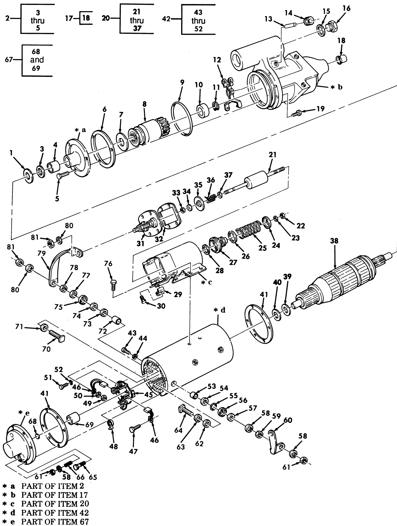
Figure 45. Starter Motor Assembly.
