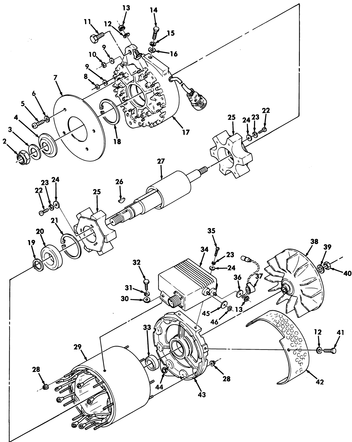
Figure 43B. Alternator, 100 AMP (NIEHOFF).
