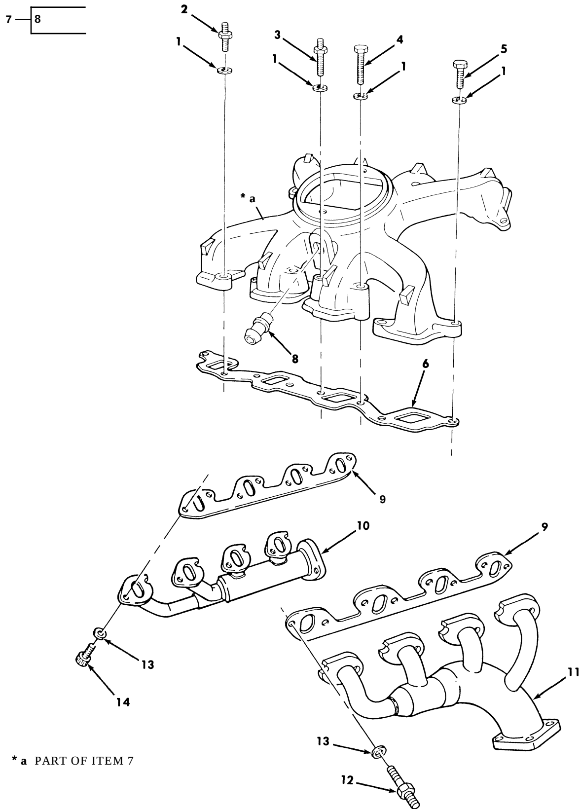
Figure 8. Air Intake and Exhaust Manifolds.
