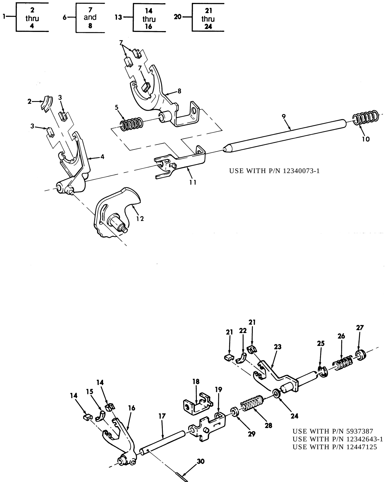
Figure 132. Transfer Shift Mechanisms.
