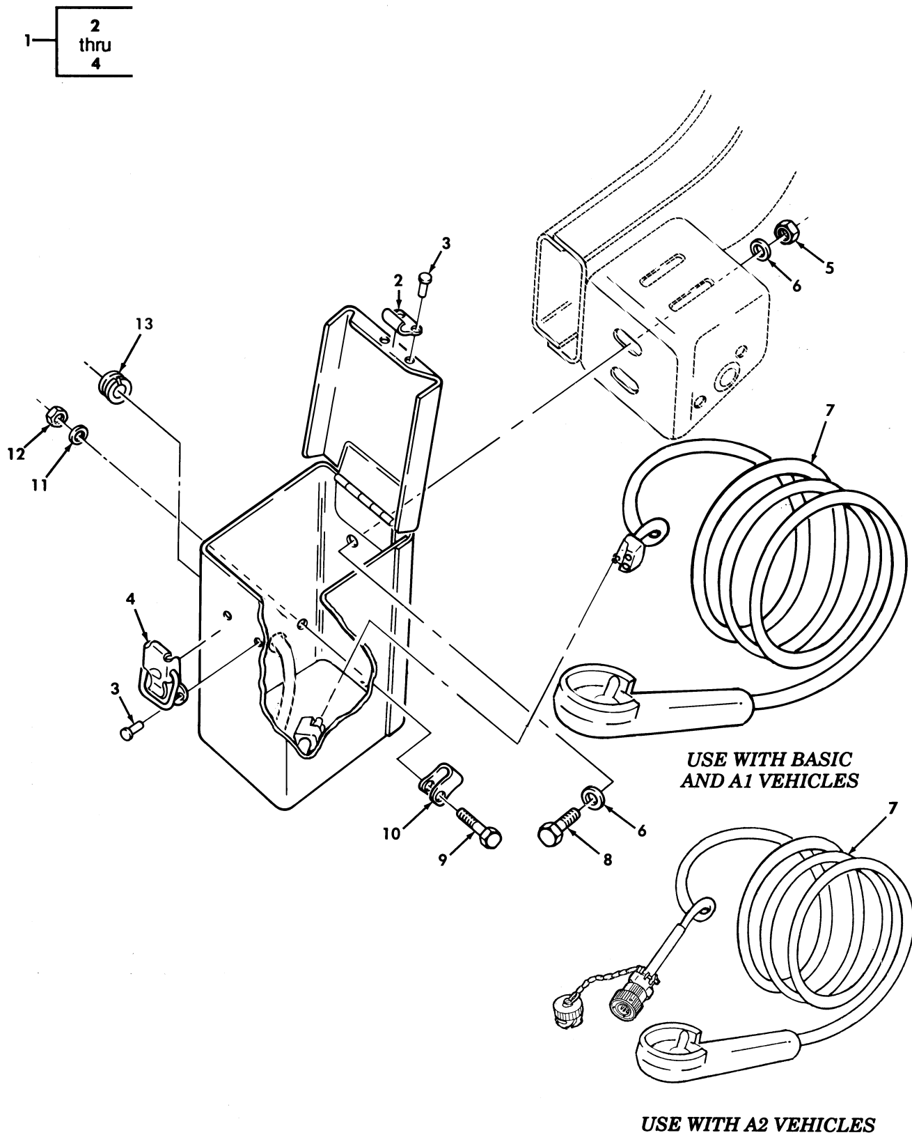
Figure 315. Winch Control, Storage Box, and Mounting Hardware.
