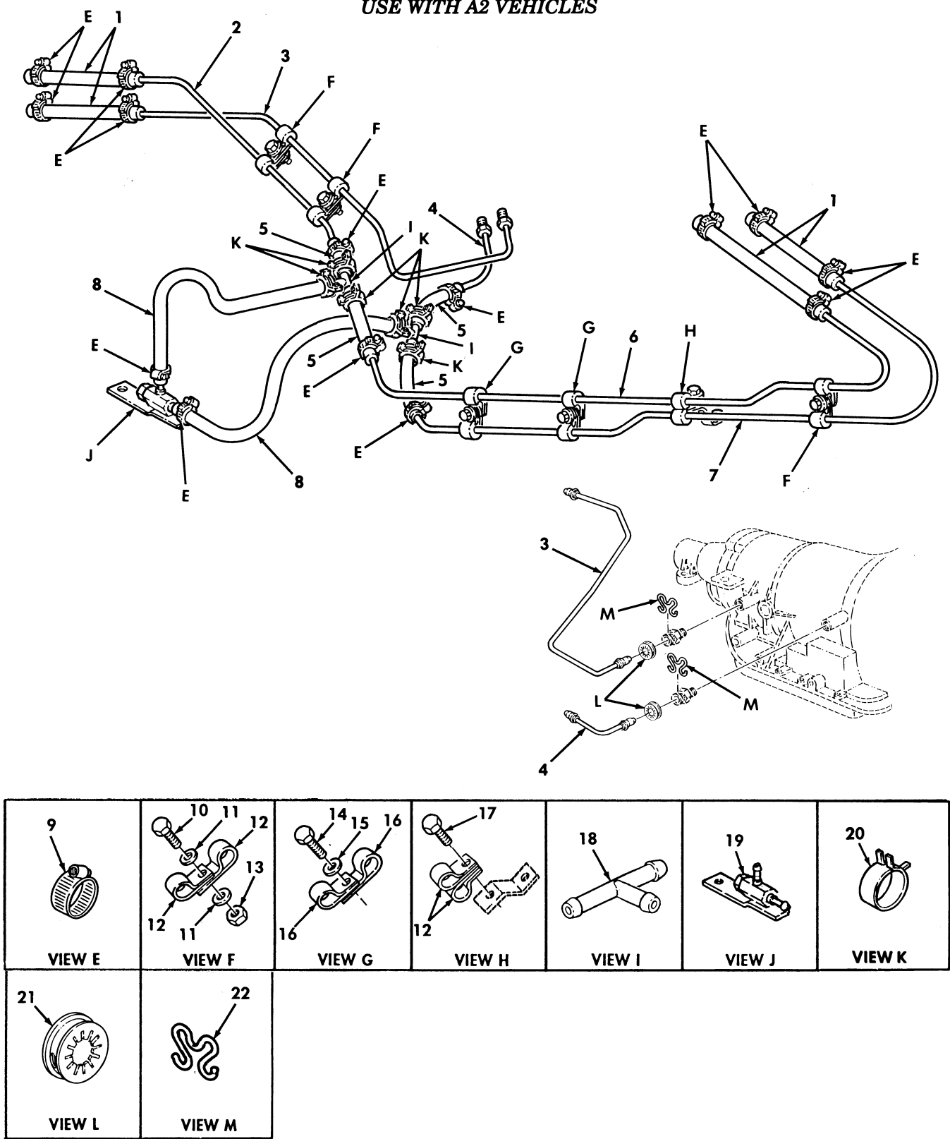
Figure 125. Transmission/Transfer Cooling Lines.
