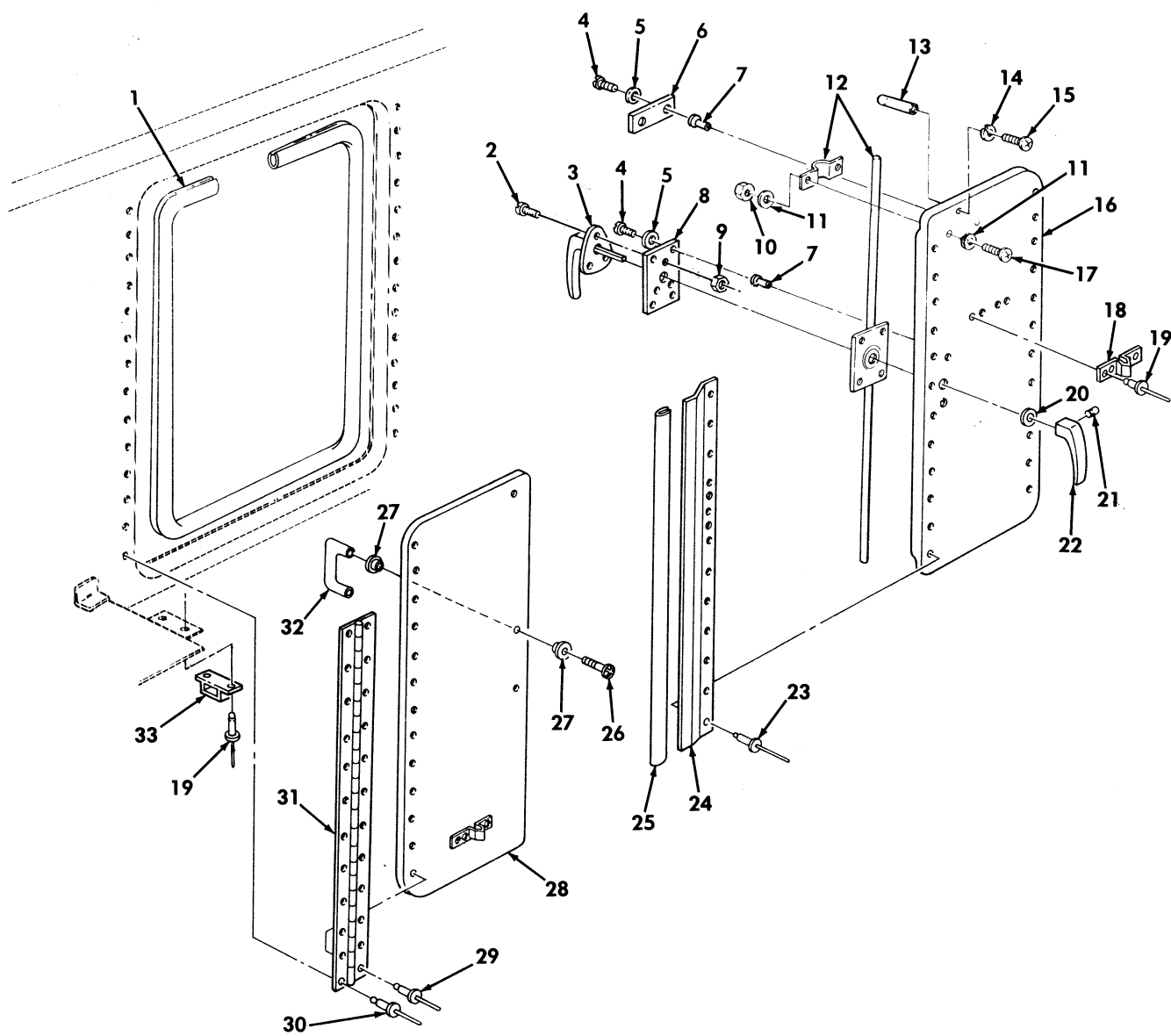
Figure 214. Bulkhead Doors and Related Parts, M997, M997A1, and M997A2 Ambulance.
